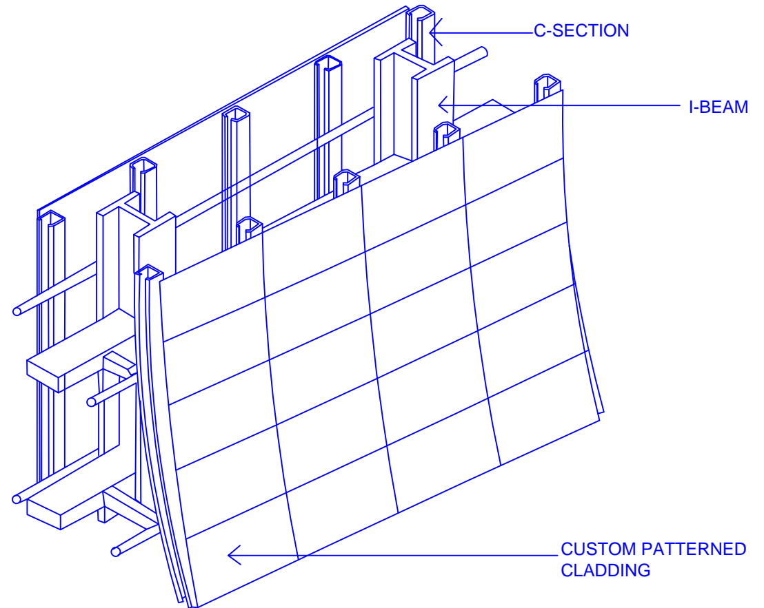
ISOMETRIC OF TITANIUM CLADDING WALL
