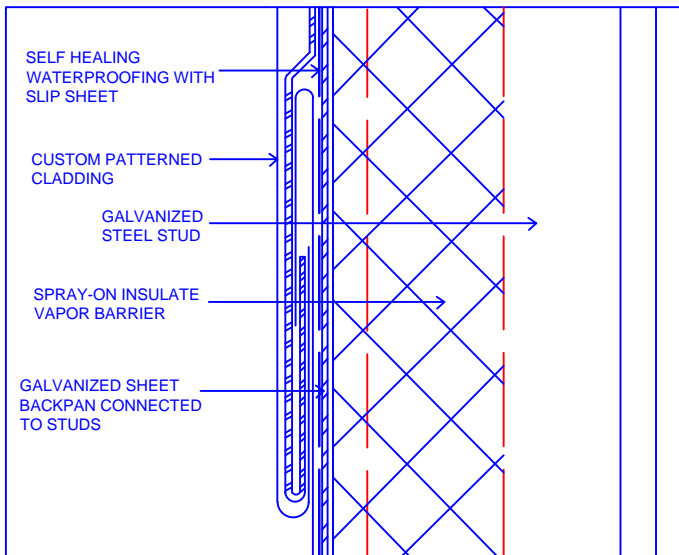
SECTION OF TITANIUM CLADDING WALL
